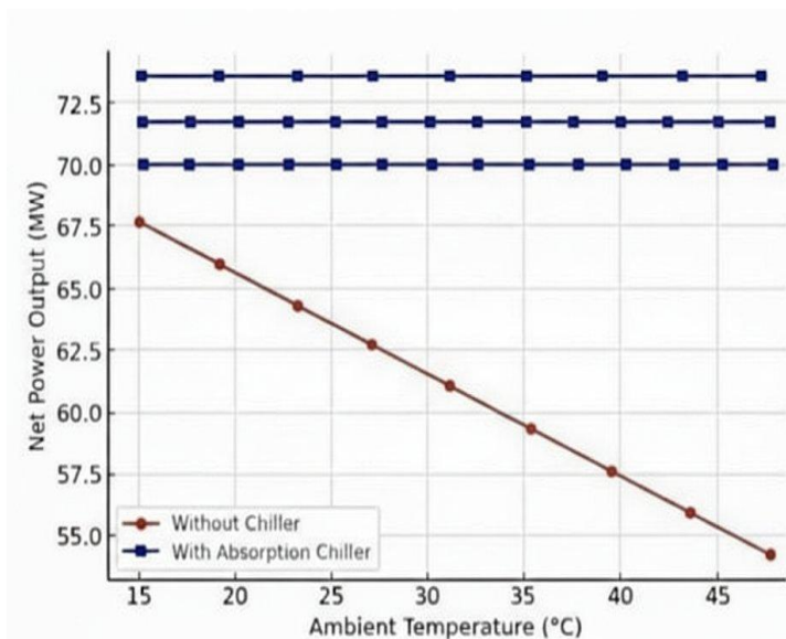
Figures 4 depict the effect of ambient temperature on power output
