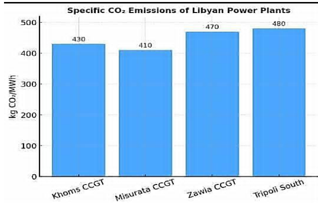
Figure (7). Specific CO 2 Emissions of Libyan Power Plants
