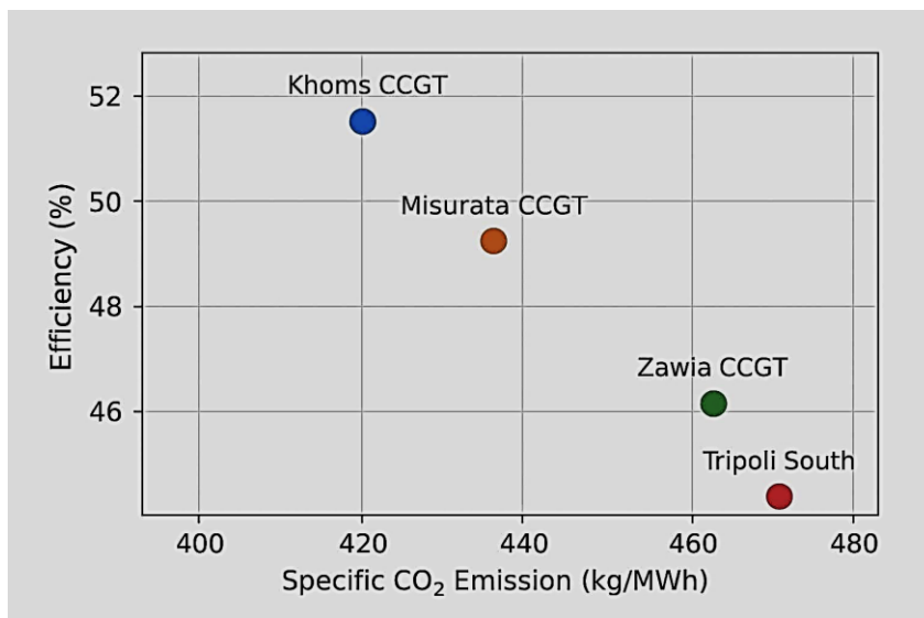
Figure (5). illustrates the relationship between efficiency and CO 2 emissions for each power plant
