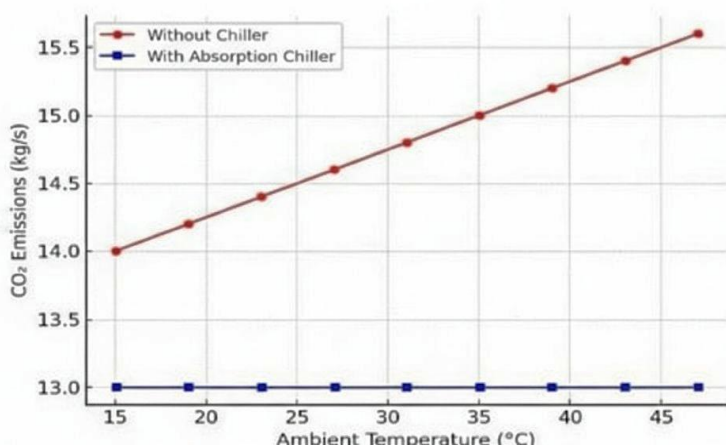
Figure. 3. CO 2 emissions with without absorption chiller.
