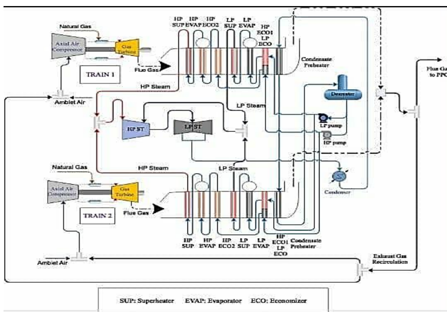
Figure (1) Combined cycle gas turbine (CCGT) power plants [9]
